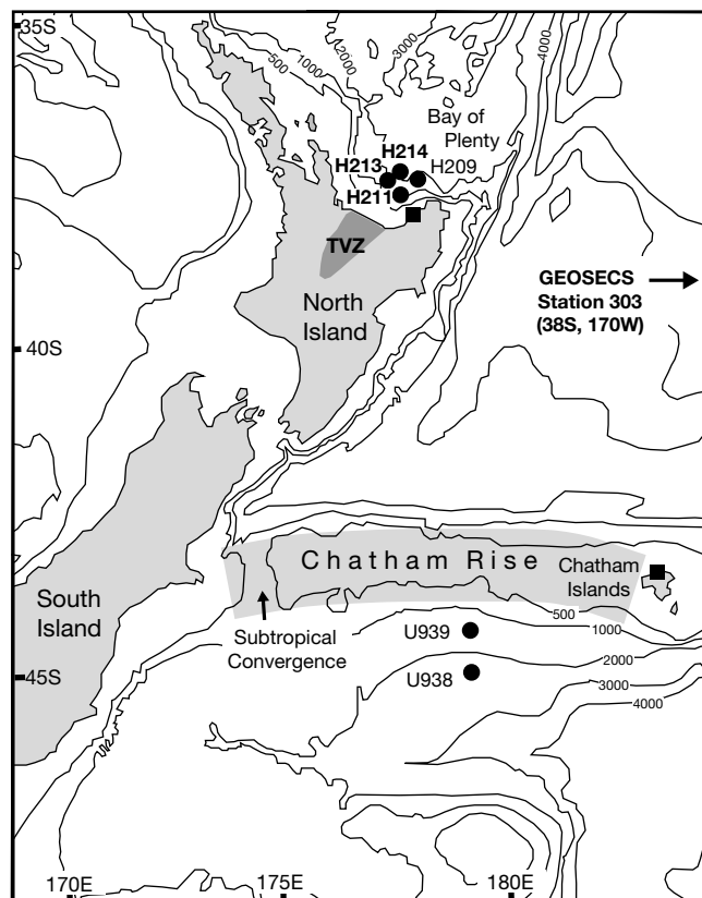
Figure 1 Locations of sediment cores and modern samples used in this study. Deep-sea sediment cores are from the Bay of Plenty and south of Chatham Rise (solid circles), and modern pre-bomb samples (solid squares) are coastal samples from the northeast North Island and the Chatham Islands. We note that the subtropical convergence (STC), which separates subtropical waters in the north from subpolar waters to the south, lies north of the southern Chatham Rise core sites. It is well established that on the Chatham Rise, the STC did not move from this position in the last glaciation 31 , in contrast to other parts of the Southern Ocean. The Taupo volcanic zone (TVZ) is the source of the tephras. Latitude of GEOSECS Station 303 (radiocarbon profile shown in Fig. 3) is indicated by arrow.
